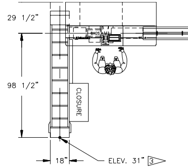
Left-hand variety bagger with front discharge
