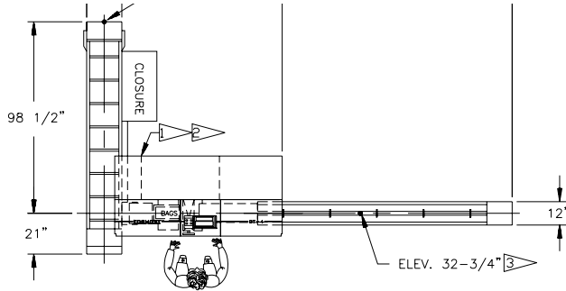
Left-hand variety bagger with rear discharge
