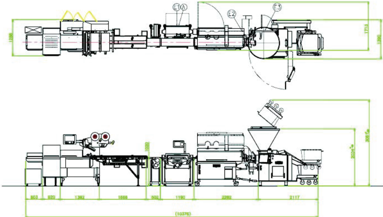
Wrapper layout with Reiser Vemag
